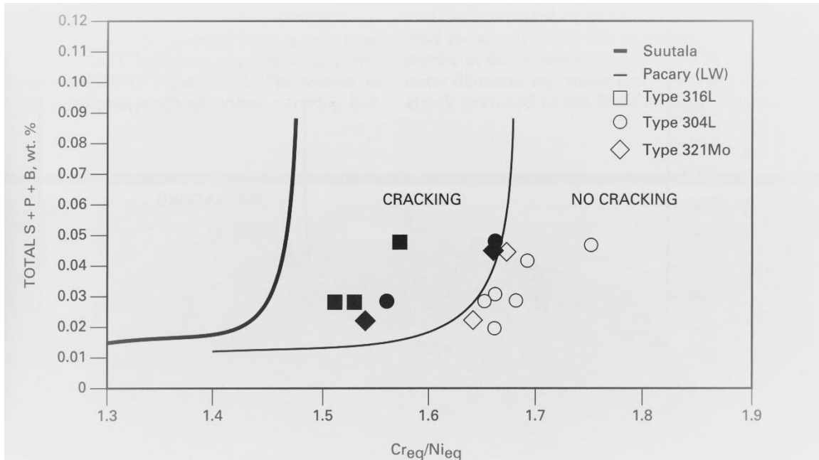
Figure 1. Modified Suutala diagram showing crack sensitivity of 304L, 316L, and 321Mo. Data shows 316L is prone to cracking with pulsed laser welding.
